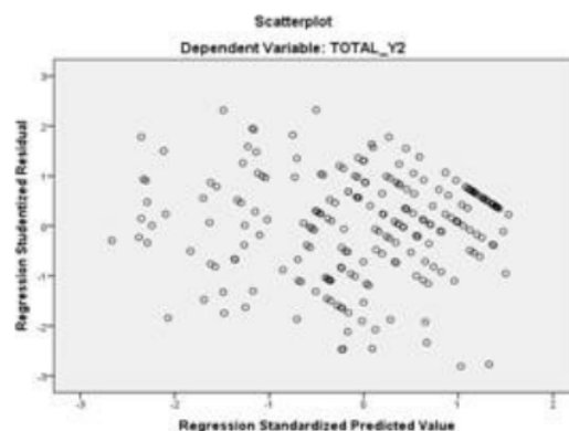
Figure 3. Heteroskedastisitas Test Results
